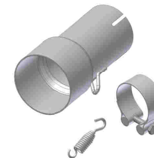
INLET PIPE 00.73.KU.00006
