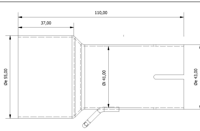
INLET PIPE 00.73.KU.00001
