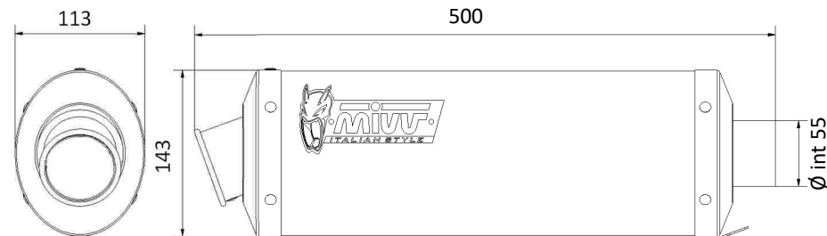
Oval Inox ( Destro / Right ) Cod.: 00.73.KU.001.SX2
