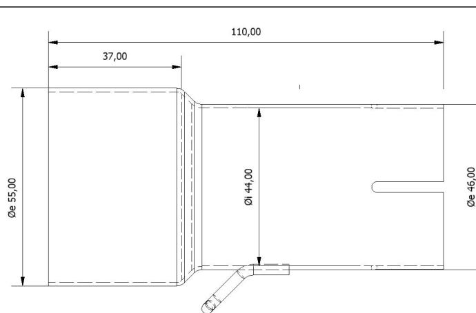
INLET PIPE 00.73.KU.00002
